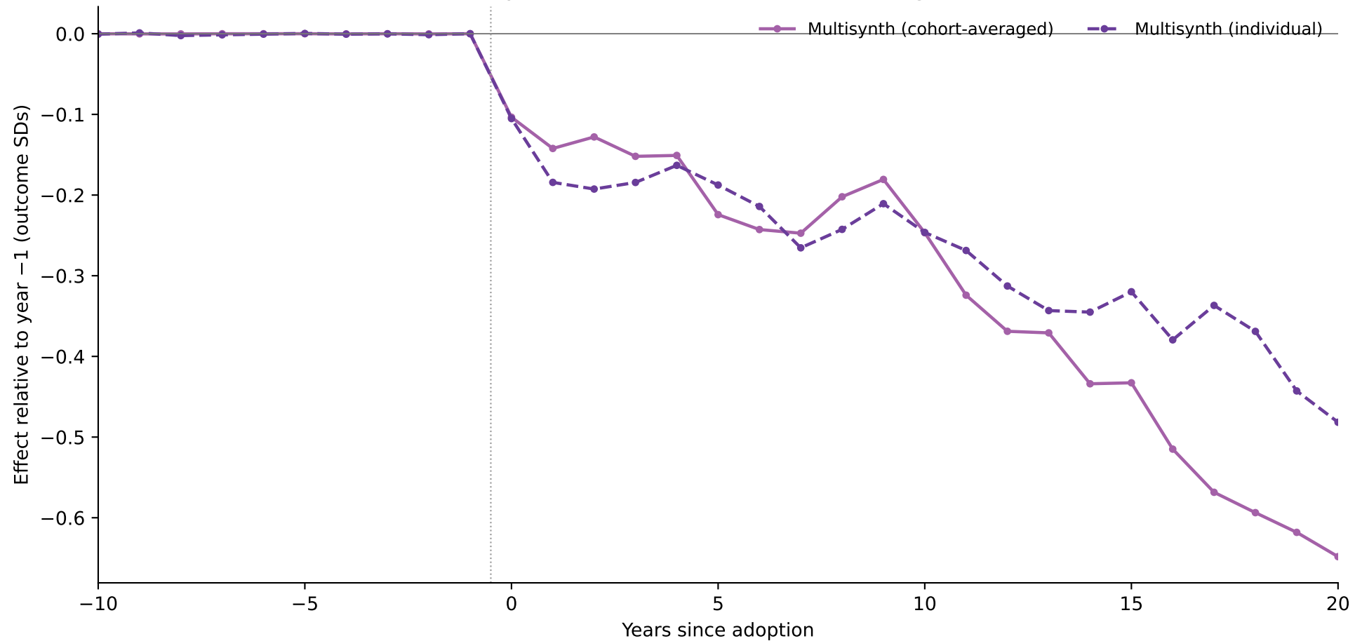
Multisynth: individual versus cohort-averaged fits
